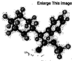
Laguna Design/Getty Images The molecular model of Ritalin.
